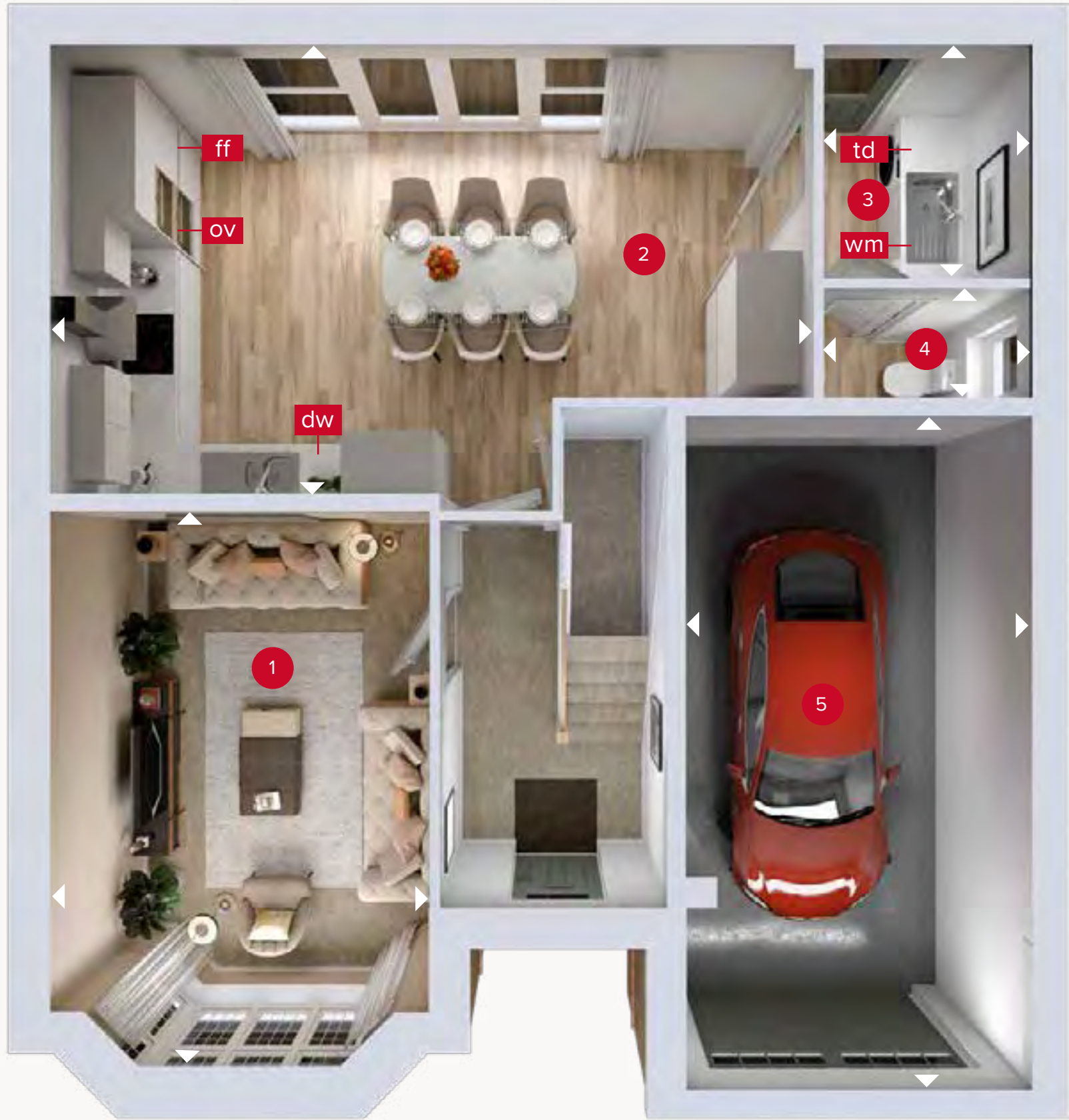
GROUND FLOOR
